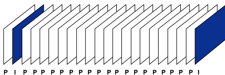
Static scene
